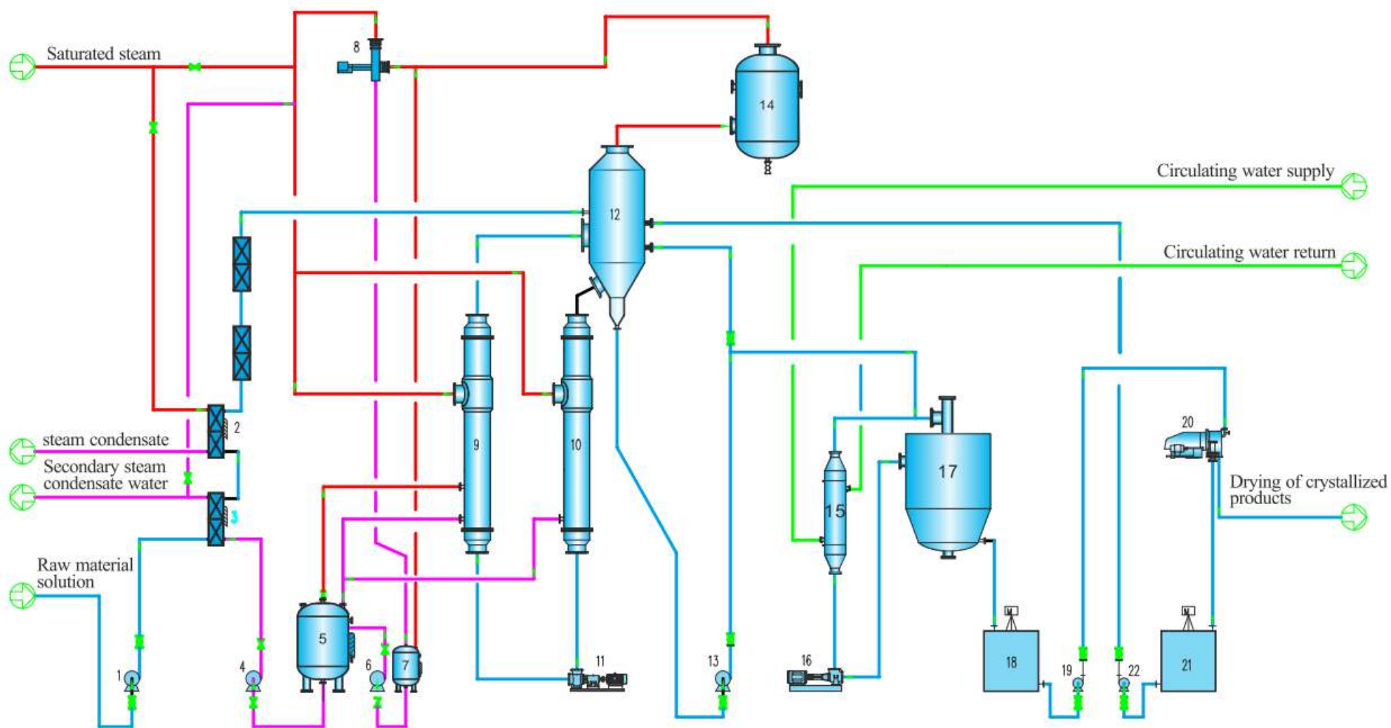
1. Raw material pump 2, steam preheater 3, condensate water preheater 4, condensate water pump 5, condensate water tank 6, liquid accumulation pump 7, liquid accumulation tank 8, compressor 9, heating chamber A 10, heating chamber B 11, evaporation circulation pump 12, evaporator 13. Discharge pump 14, demister 15, crystallization external cooler 16, cooling crystallization circulation pump 17, cooling crystallizer 18, crystallization buffer tank 19, crystallization discharge pump 20, centrifuge 21, centrifugal mother liquor tank 22, centrifugal mother liquor pump
